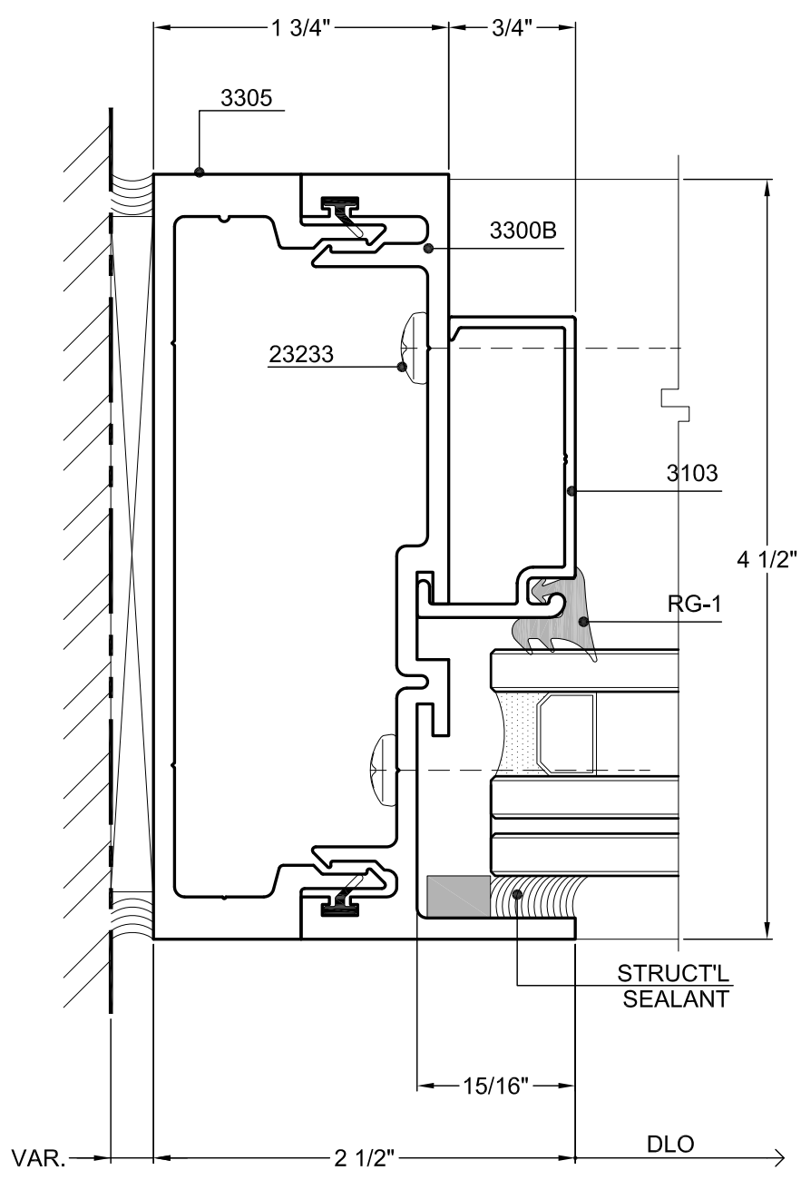
④ TYPICAL JAMB
