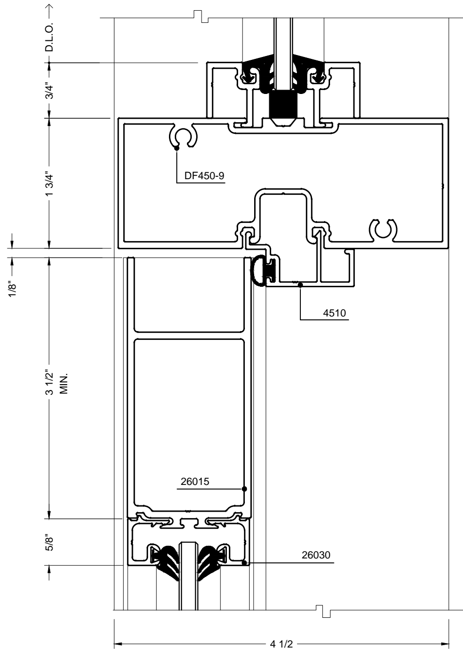
(41) MS DOOR HEADER W/ TRANSOM (STANDARD) OFFSET PIVOT & BUTT HINGE FOR CONTINUOUS GEAR HINGE REFER TO 30.1
