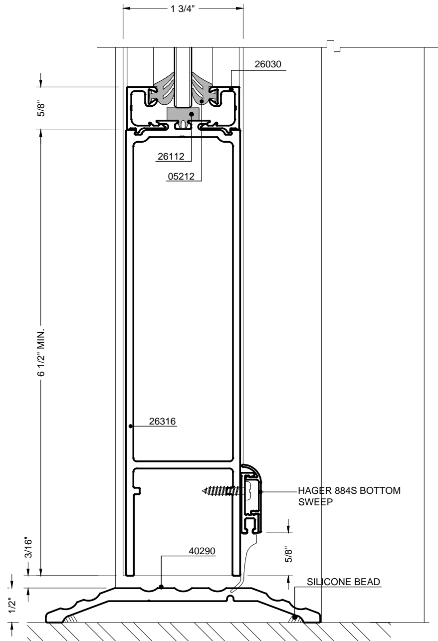
42 WS BOTTOM RAIL (STANDARD)
