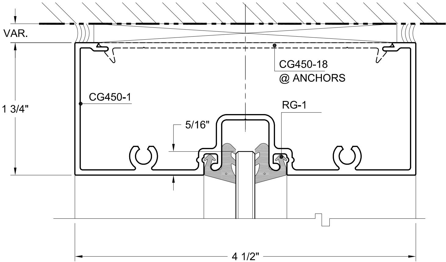
10 TYPICAL HEAD
