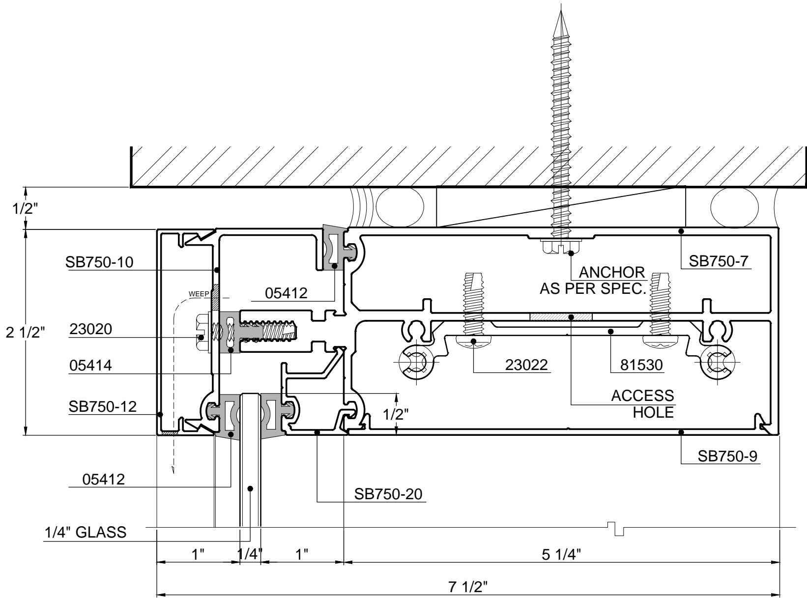
10C ALTERNATE HEAD (SCREW ANCHOR) 1/4" GLASS OPTION
