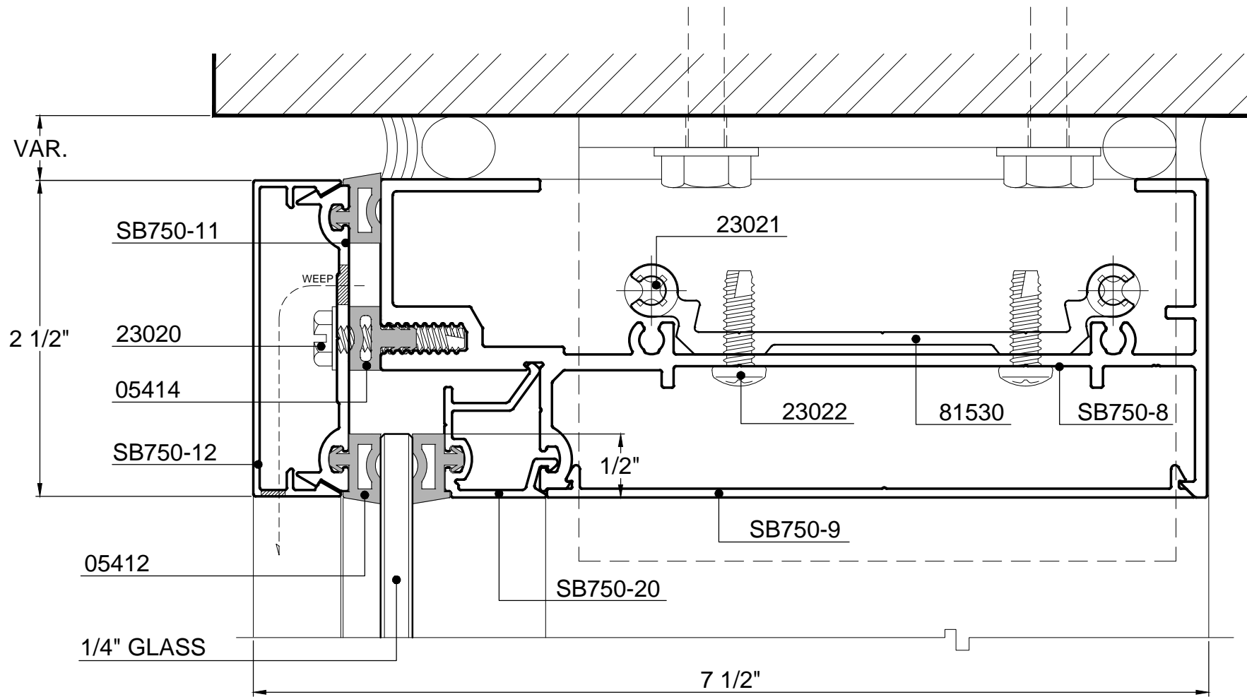
10B OPEN BACK HEAD (F&T ANCHOR) 1/4" GLASS OPTION
