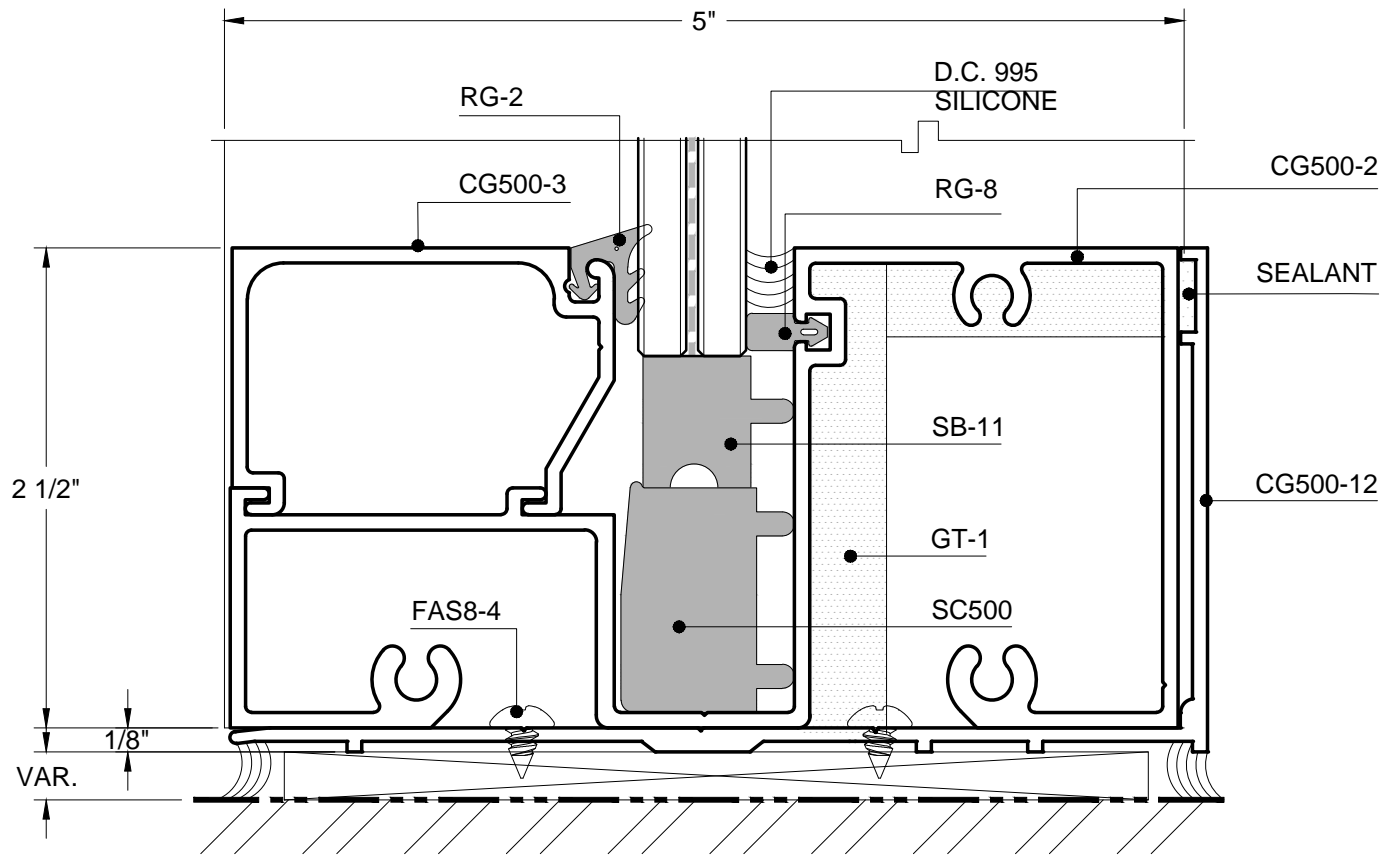
(12) TYPICAL SILL
