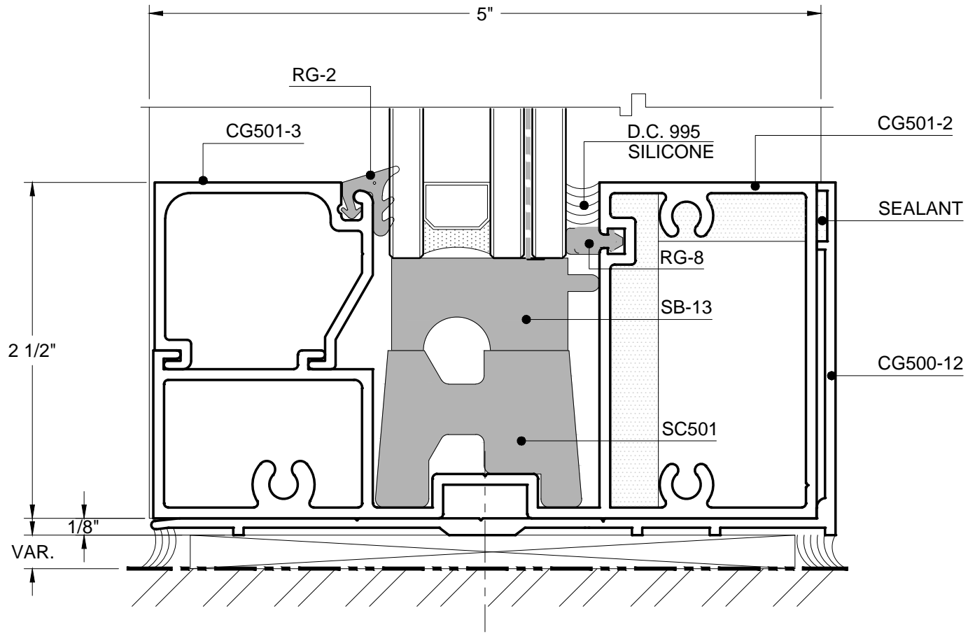
12 TYPICAL SILL
