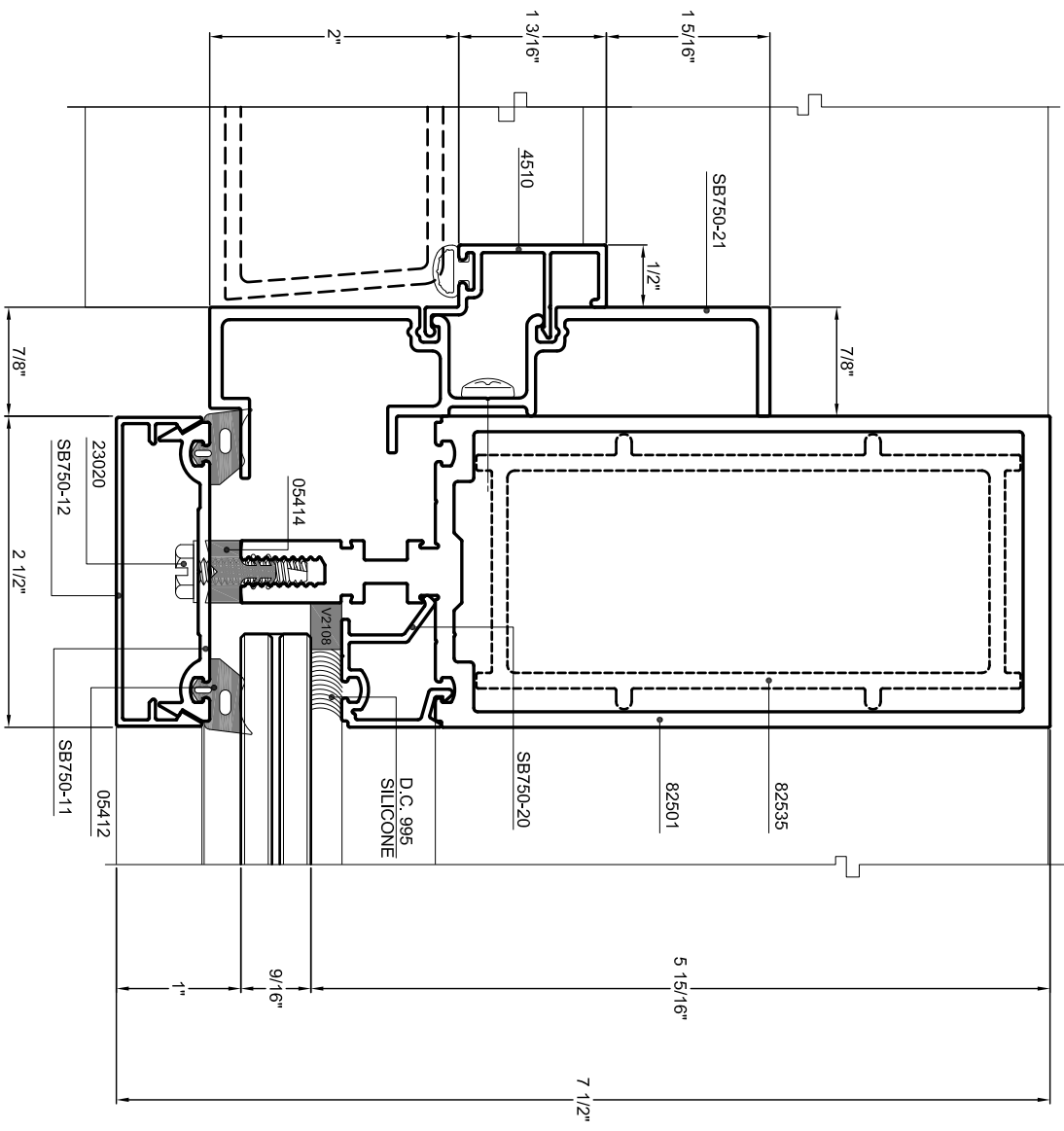
41B DOOR JAMB INTERFACE WITH SUB-FRAME
