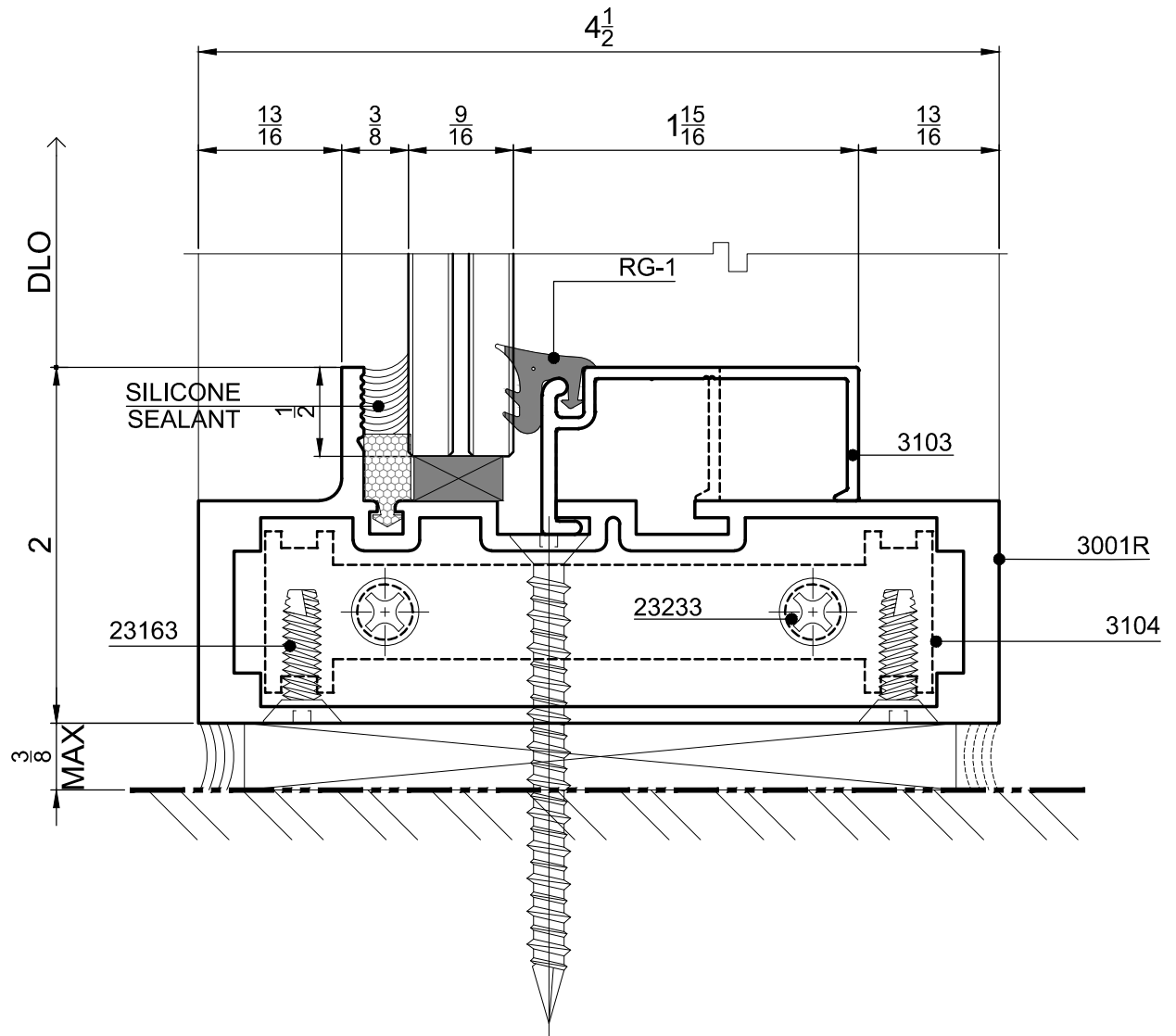
3 SILL DETAIL
