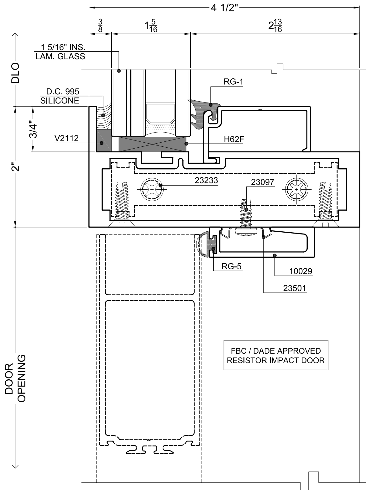
8 DOOR HEAD DETAIL
