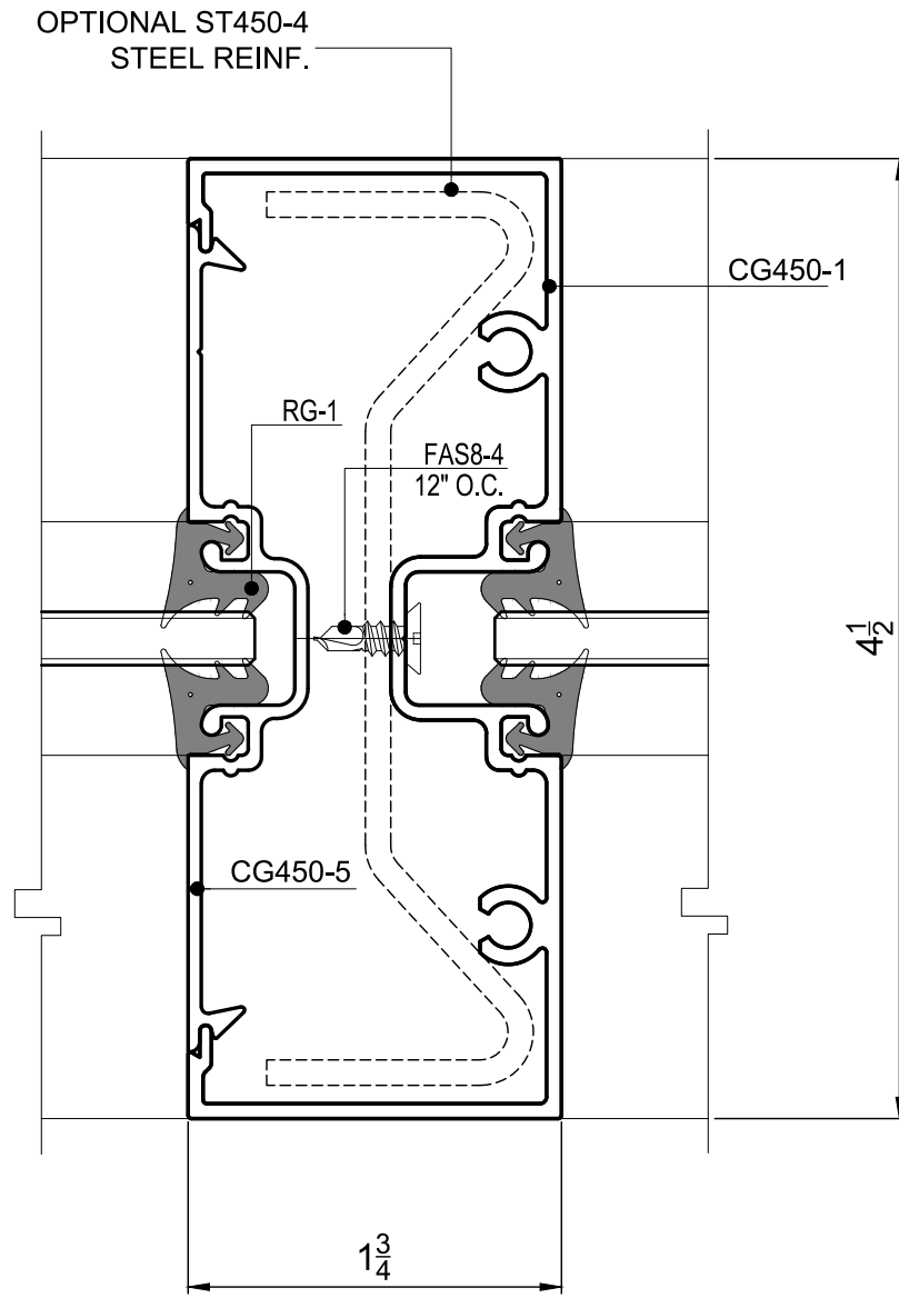
5 LIGHT MULLION
