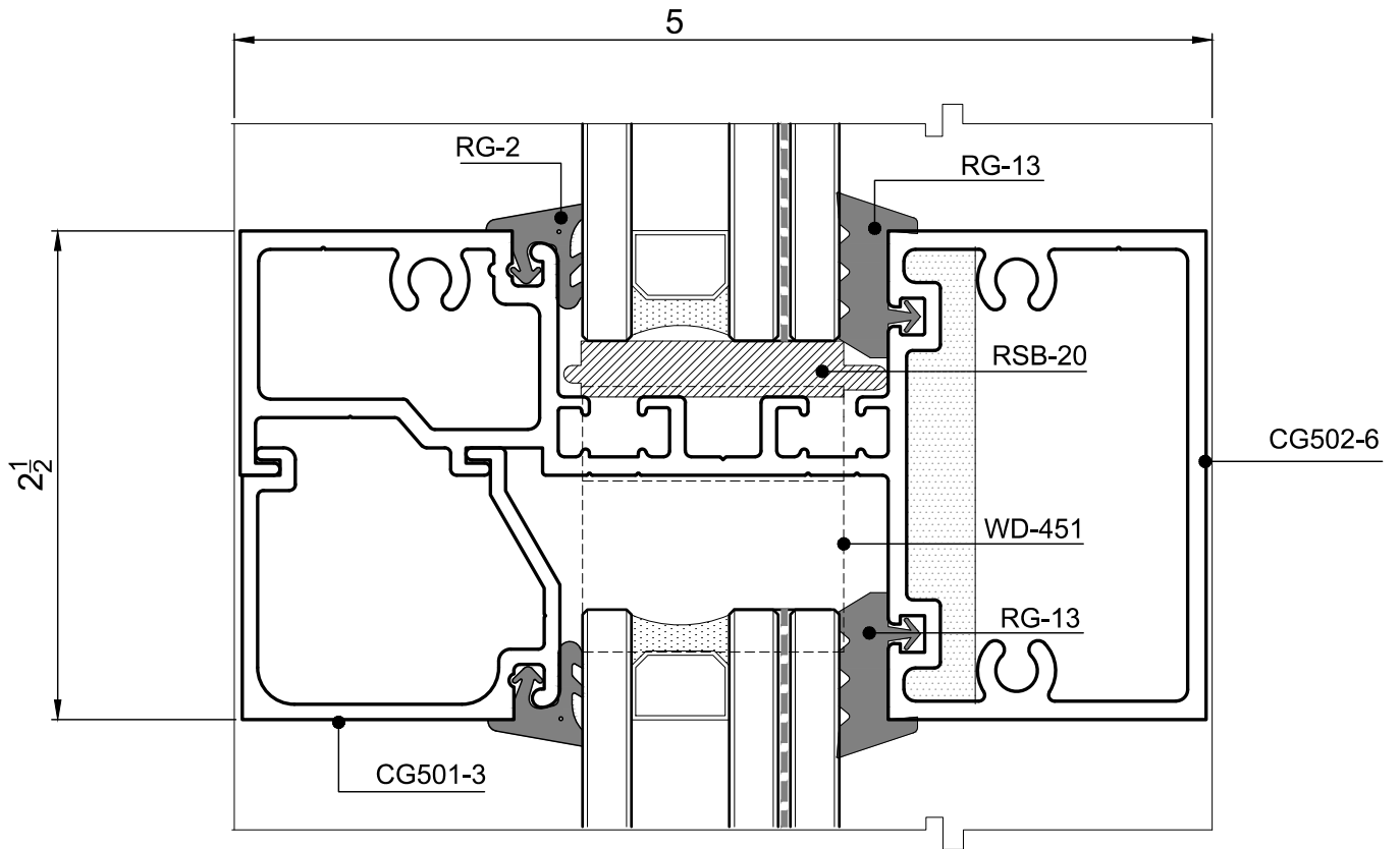
② ALT. INTERMEDIATE HORIZONTAL NON-THERMAL
