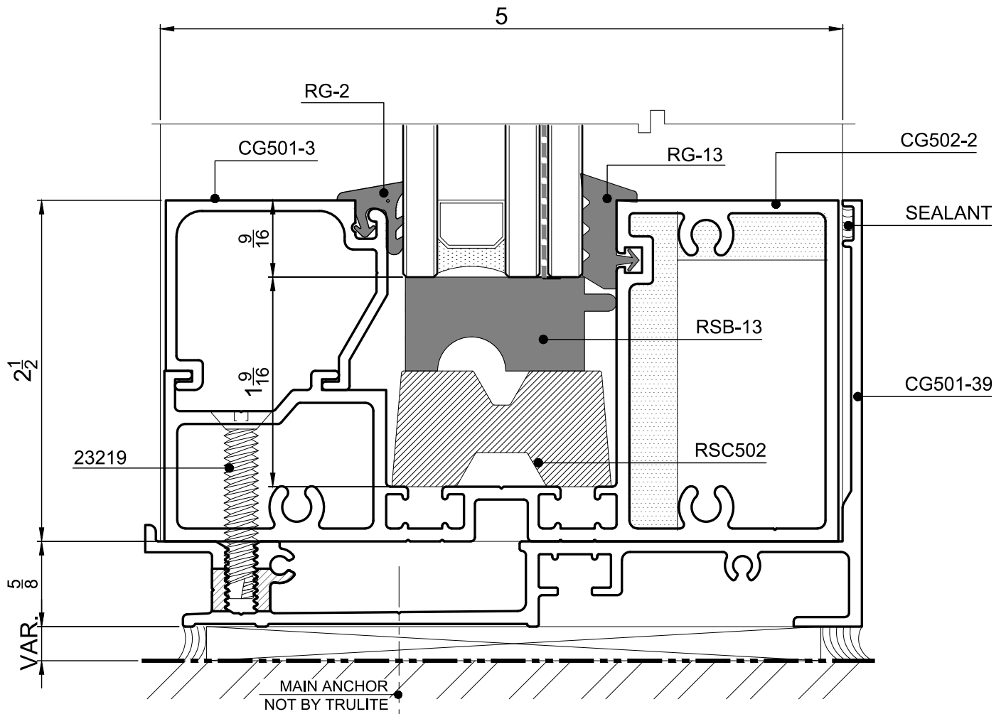
4 TYPICAL SILL NON-THERMAL
